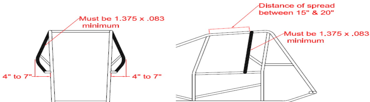
#1 Support Bar
